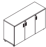
Pre-laminated storage (three door unit) Height - 700 Width - 1050 / 1200 Depth - 425
